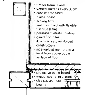
⑫ Floor/wall structure in damp areas in a half-timbered building
